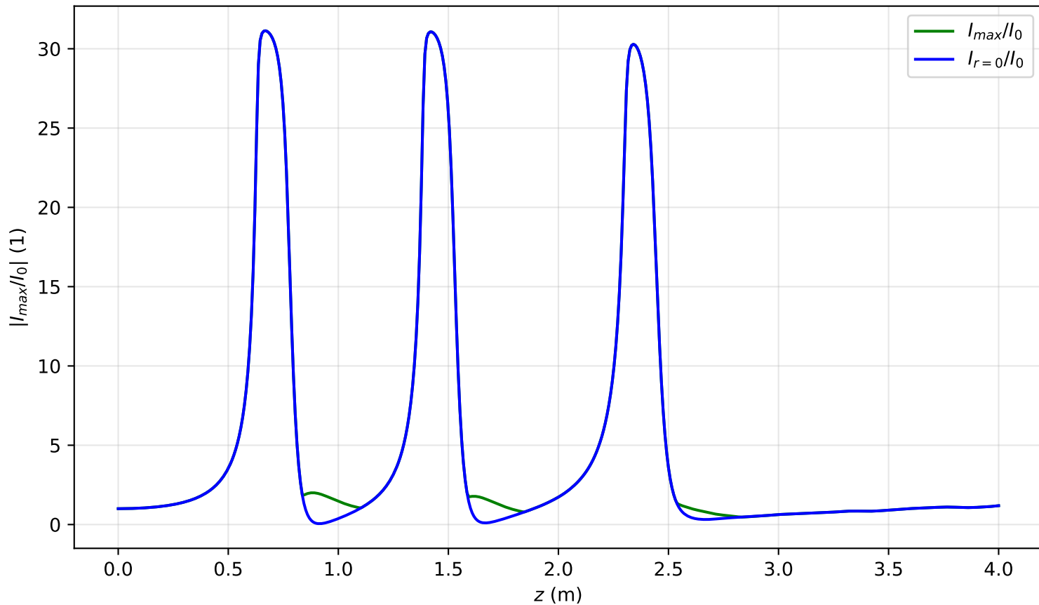
I_{max}(x = 0, y = 0, z)/I_0 , \text{Pin}=3.5\text{Pcr} , artificial time
